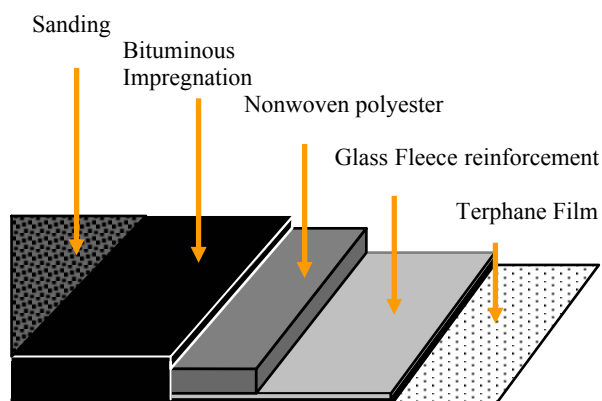
Figure 1: Typical cross-section
